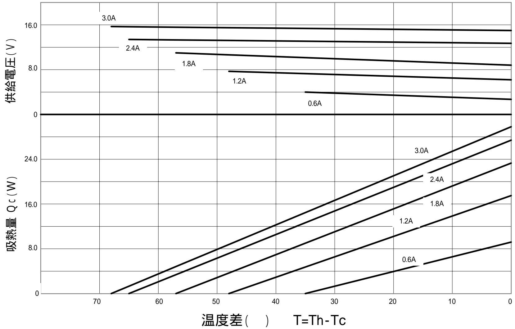
FPH1 - 12703M 特性図(Th=27 )
